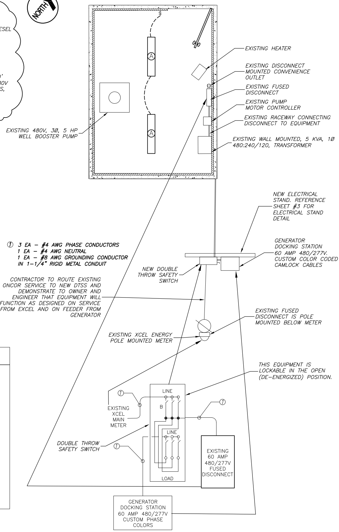
DIAGRAM FOR GENERATOR DOCKING STATION UPGRADE ON WELL #8
